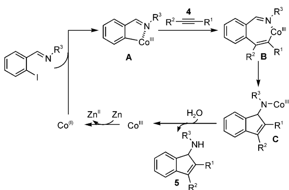
Scheme 3. Proposed mechanism for the Co-catalyzed formation of indenamines.
