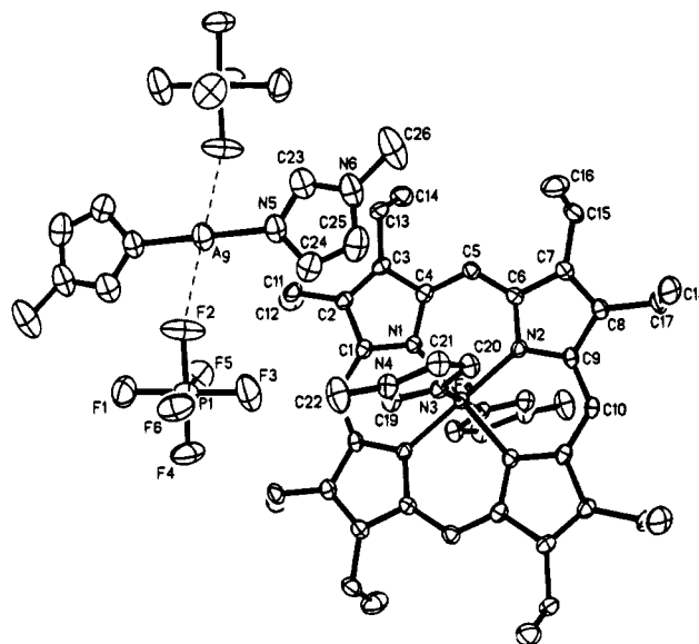
Figure 3. Structure of [Fe(OEP)(N-MeIm) 2 ][Ag(N-MeIm) 2 ][PF 6 ] 2 (50% probability thermal ellipsoids). Hydrogen atoms have been omitted for clarity. The separation of the various ions is to scale.
