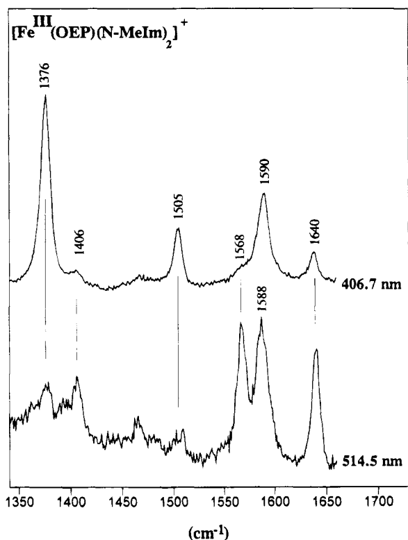
Figure 11. Resonance Raman spectra of [\text{Fe}(\text{OEP})(N\text{-MeIm})_2][\text{Ag}(N\text{-MeIm})_2][\text{PF}_6]_2 in the high-frequency region. The sample was prepared by diluting the microcrystalline specimen with 1–3% \text{Na}_2\text{SO}_4 by weight. Other conditions paralleled those given under Figures 10 and 8, with the exception that the data are shown as collected. Polarization data reported in Table 4 were obtained from a \text{CH}_2\text{Cl}_2 solution to which 500 mM free N -methylimidazole was added.
