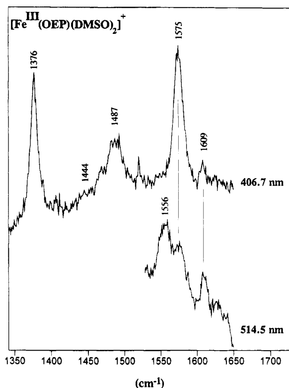
Figure 12. Resonance Raman spectra of [\text{Fe}(\text{OEP})(\text{DMSO})_2][\text{PF}_6] in the high-frequency region obtained with 406.7- and 514.5-nm excitation and prepared as described in the legend to Figure 11. Polarization data reported in Table 4 were obtained from a 1:1 \text{CH}_2\text{Cl}_2 :DMSO solution. Data are shown as collected.
