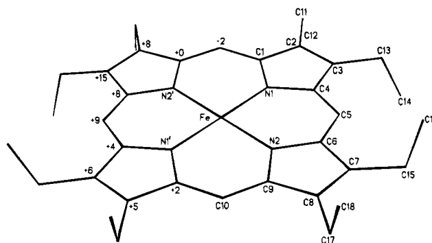
Figure 4. Drawing showing the perpendicular displacement of each atom from the least-squares plane through the 24 atoms of the porphyrin core of [Fe(OEP)(N-MeIm) 2 ][Ag(N-MeIm) 2 ][PF 6 ] 2 . Although the Fe(N por ) 4 unit is rigorously planar, the porphyrin core is distorted so that two adjacent pyrrole rings (left rear and left front) are slightly tilted up and two (right rear and right front) are slightly tilted down.
