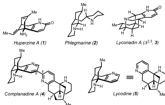
Figure 1. Selected Lycopodium alkaloids.
