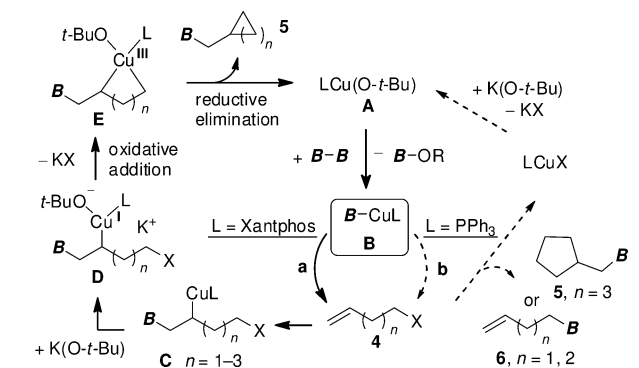
Scheme 9. Proposed Mechanism for the Copper(I)-Catalyzed Borylative Cyclization
