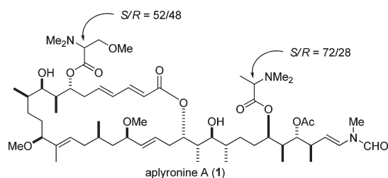
Figure 1. Structure of aplyronine A ( 1 ).
