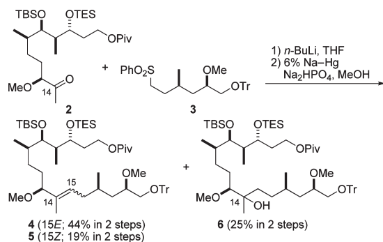
Scheme 1. Our Previous Work
