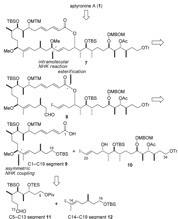
Scheme 2. Second-Generation Retrosynthetic Analysis of Aplyronine A ( 1 )
