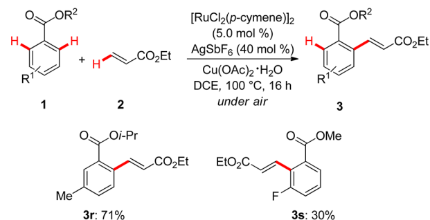
Scheme 4. Intramolecular Competition Experiments
