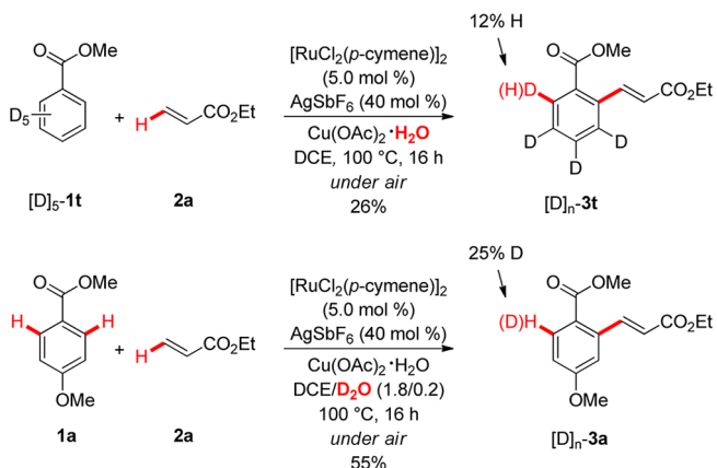
Scheme 6. Oxidative Alkenylation with Isotopically Labeled Substrate or Cosolvent
