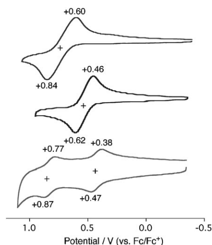
Figure 3. Cyclic voltammograms of fused oligothiophenes of 6a (top), 6b (middle), and 6c (bottom). Measurement conditions: n\text{Bu}_4\text{NPF}_6 (0.1 M) in o -dichlorobenzene; scan rate 50 \text{ mV s}^{-1} .
