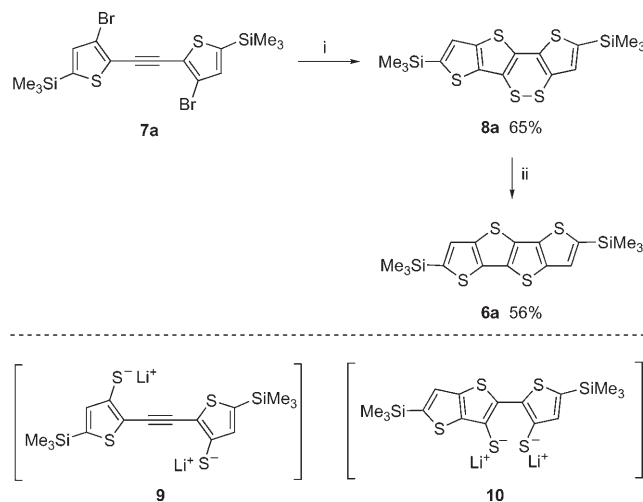
Scheme 2. Synthesis of tetrathienoacene 6a and the plausible intermediates. Reagents and conditions: i) 1) t\text{BuLi} , THF; 2) \text{S}_8 (3.0 mol amt.); 3) \text{K}_3[\text{Fe}(\text{CN})_6] , 1 N aq. NaOH. ii) Cu nanopowder, 300 °C.
