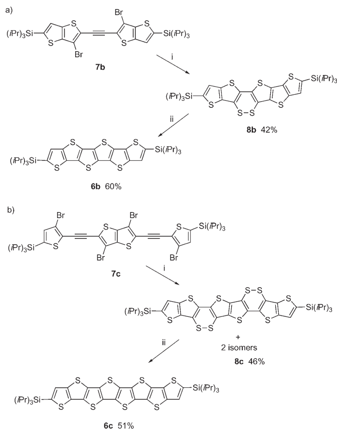
Scheme 3. Synthesis of a) hexathienoacene 6b and b) octathienoacene 6c . Reagents and conditions: i) 1) t BuLi, THF; 2) S_8 (3.0 mol amt.); 3) K_3[Fe(CN)_6] , 1 N aq. NaOH. ii) Cu nanopowder, 300–340 °C.
