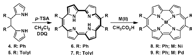
Scheme 1. Syntheses of 6–9
