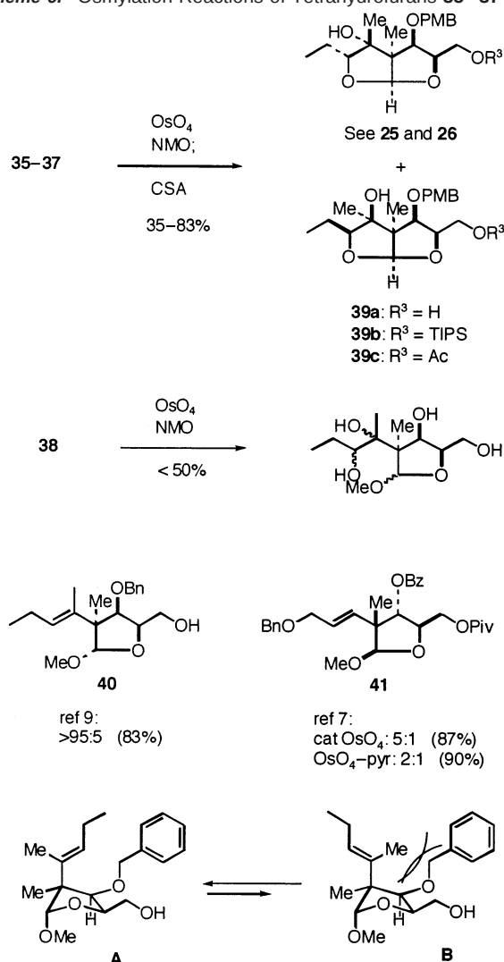
Scheme 6. Osmylation Reactions of Tetrahydrofurans 35–37
