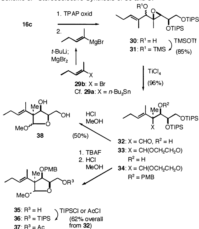
Scheme 5. Stereoselective Synthesis of 36 and 37
