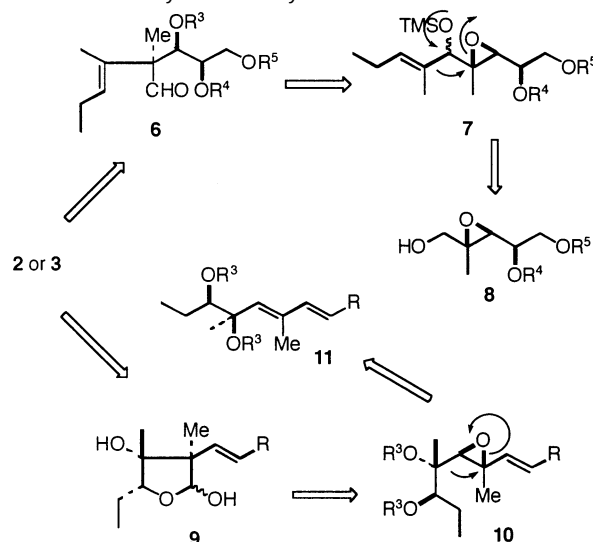
Scheme 2. Retrosynthetic Analysis
