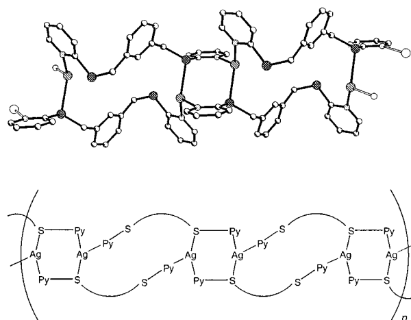
Fig. 4 Perspective view (top), with hydrogens omitted, and schematic representation (bottom) of a section of the extended polymeric structure of complex 3 . Nitrate anions are not shown.
