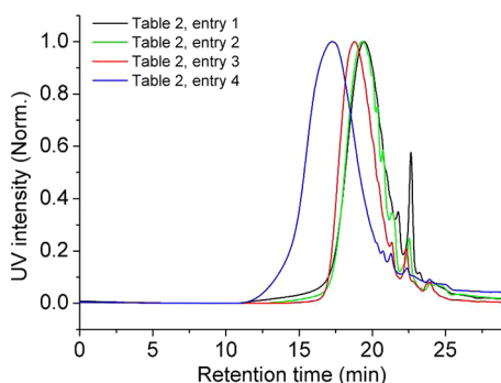
Figure 1. THF SEC trace monitored using a UV detector at 254 nm.
