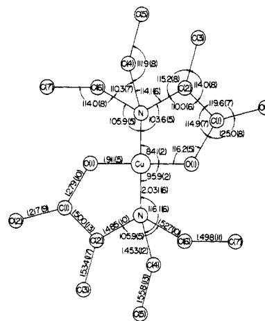
Figure 2. Bond distances and angles in the bis( N,N -diethyl- \alpha -alaninato)copper(II) molecule.
