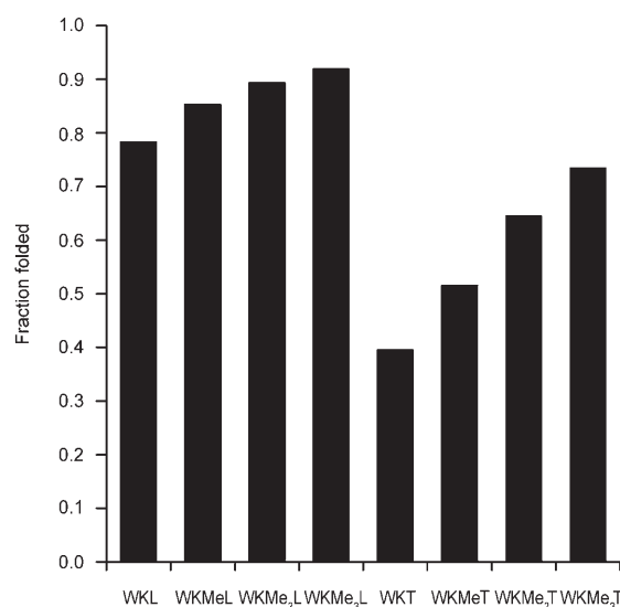
Figure 7. Fraction folded (based on glycine splitting) of WK(Me) n T and WK(Me) n L ( n=0-3 ) \beta -hairpins.
