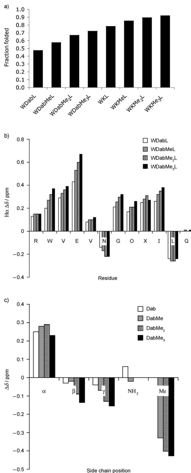
Figure 11. a) WDab(Me) n L and WK(Me) n L fraction folded comparison. b) WDab(Me) n L H α shifts relative to random coil values. Glycine shifts reflect the splitting. c) WDab(Me) n L side chain upfield proton shifts relative to random coil values.
