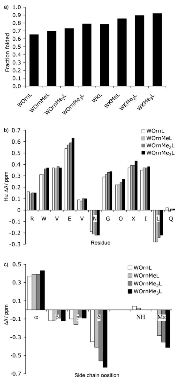
Figure 9. a) WOrn(Me) n L and WK(Me) n L fraction folded from the glycine splitting. b) WOrn(Me) n L H_\alpha shifts relative to random coil values. Glycine shifts reflect the splitting. c) WOrn(Me) n L side chain upfield proton shifts relative to random coil values.
