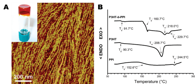
Figure 2. (A) AFM phase image of 3b drop-casted from CHCl 3 ( [3b]_0 = 10 mg mL -1 ) onto a Si wafer (film thickness = 80 nm). Inset: Photograph showing gelation behavior of 3c in CHCl 3 (the critical gelator concentration was determined to be 15 mg mL -1 at 25 °C). (B) DSC thermograms of (top) 3c , (middle) P3HT ( M_n = 8.2 kDa), and (bottom) a homopolymer of 2 ( M_n = 17 kDa) (rate = 10 °C min -1 ).
