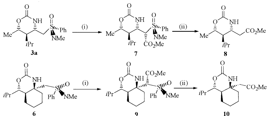
Scheme 3. (i) 1. 2.2 equiv. of n BuLi, THF, -78^\circ\text{C} ; 2. \text{ClCO}_2\text{Me} , -78^\circ\text{C} , 4 h. (ii) Ra-Ni, THF, \text{H}_2\text{O} , 22^\circ\text{C} , 8 h
