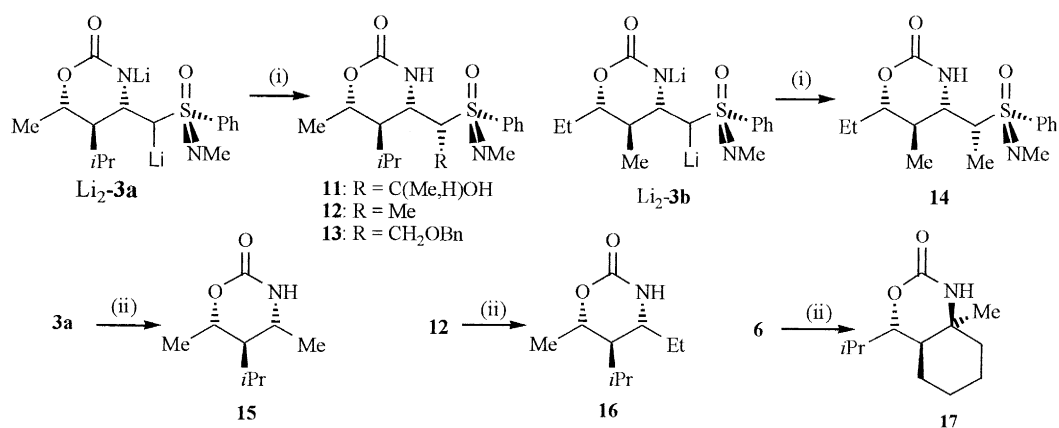
Scheme 4. (i) MeCHO, MeI or \text{BnOCH}_2\text{Cl} , THF, -78^\circ\text{C} . (ii) Ra-Ni, THF, \text{H}_2\text{O} , 22^\circ\text{C} , 5–18 h
