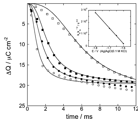
Figure 6. Difference, \Delta Q , between the pristine charge transient and the immediately subsequent one on a Hg-supported 5 − SAM in aqueous 0.1 M TMACl. The charge transients were obtained by stepping from E_i = -0.75 V to E_f = -1.60 (open squares), -1.65 (solid squares), -1.70 (solid circles), and -1.80 V (open circles). The solid curves were calculated from the model described in the text for n = 2 , NF = -2.5 \mu\text{C cm}^{-2} and for different values of the kinetic parameter k_R k_N^{1/2} . This parameter is plotted against the final potential E_f in the inset.
