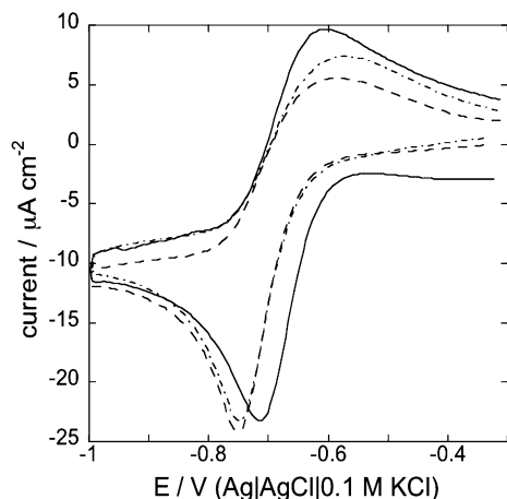
Figure 7. Cyclic voltammogram of 1 \times 10^{-4} M Eu(III) in 0.1 M KCl on bare mercury (solid curve) and on mercury coated with a 5+ (dashed curve) and a 5- SAM (dash-point curve). Scan rate: 50 mV/s.
