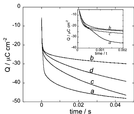
Figure 5. Charge vs time curves obtained by stepping from E_i = -0.750 to -1.80 V on newly formed Hg-supported SAMs of 5 − (curves a and b ) and of 5 − (curves c and d ), in aqueous 0.1 M TMACl; a and c were obtained from pristine potential steps, b and d from the immediately subsequent steps. The inset shows the initial portion of the four charge transients, to point out the sigmoidal shape of curve a .
