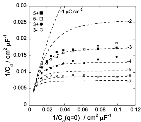
Figure 2. Dashed curves are 1/C_d vs 1/C_d(q = 0) plots calculated from the Gouy–Chapman theory for the q values reported on each curve. The solid squares, open squares, solid circles, and open circles are experimental values of 1/C_d against the corresponding 1/C_d(q = 0) values for Hg-supported SAMs of 5+, 5-, 3+, and 3-, respectively, in aqueous KCl of concentration 0.1, 5 \times 10^{-2} , 3.2 \times 10^{-2} , 2 \times 10^{-2} , 1.3 \times 10^{-2} , 8 \times 10^{-3} , 5 \times 10^{-3} , 3.2 \times 10^{-3} , and 2 \times 10^{-3} M (from left to right). Measurements were carried out at -0.75 V for the 5+, 5-, and 3+ SAMs and at -0.95 V for the 3- SAM.
