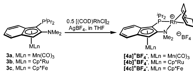
Scheme 5. Synthesis of the [(κ 2 -P,N-3a-c)Rh(COD)] + BF 4 − Complexes ( [4a-c] + BF 4 − )
