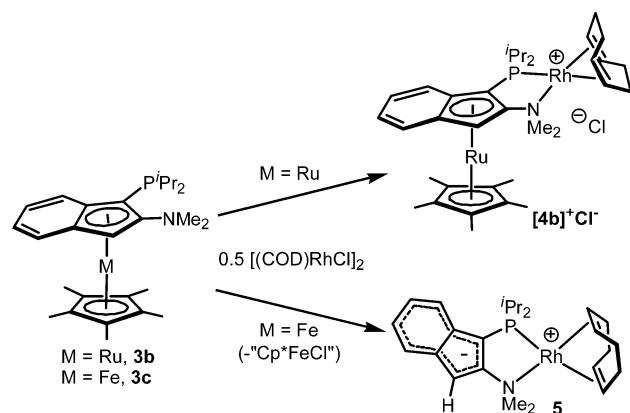
Scheme 5. Synthesis of the [(κ 2 -P,N-3a-c)Rh(COD)] + BF 4 − Complexes ( [4a-c] + BF 4 − )
