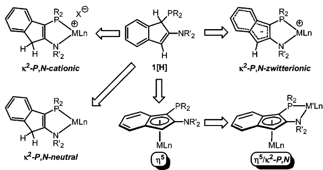
Scheme 1. Coordination Complexes Derived from P,N-Substituted Indene Ligands
