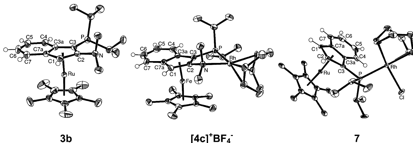
Figure 2. ORTEP diagrams for 3b , [4c] + BF 4 − , and 7 , shown with 50% displacement ellipsoids and with the atomic numbering scheme depicted. Selected hydrogen atoms, as well as the tetrafluoroborate anion in [4c] + BF 4 − , have been omitted for clarity. Only one of the two crystallographically independent molecules of 7 is shown.
