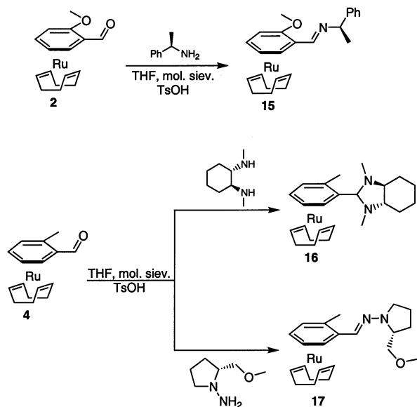
Scheme 6.
