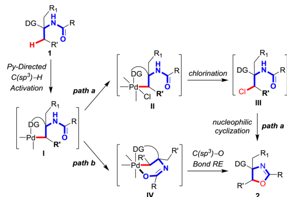
Scheme 2. Plausible Mechanism
