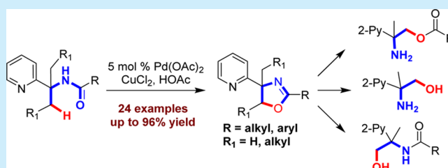
Scheme 1. Oxazoline Synthesis via C(sp 3 )–H Activation
