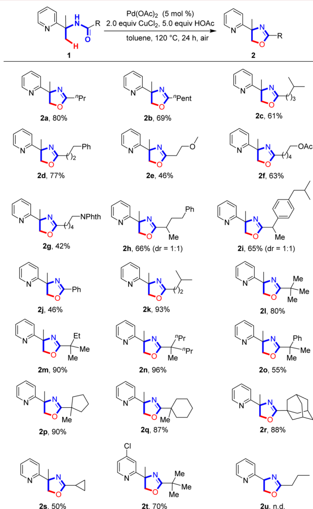
Figure 1. Pd-catalyzed annulation of methyl \text{C}(\text{sp}^3)\text{-H} bonds. Reaction conditions: 1 (0.2 mmol), \text{Pd}(\text{OAc})_2 (5 mol %), \text{CuCl}_2 (0.4 mmol) and HOAc (1.0 mmol) in toluene (2 mL) at 120 °C for 24 h under air. Isolated yields. For structure 2u , n.d. = not detected.
