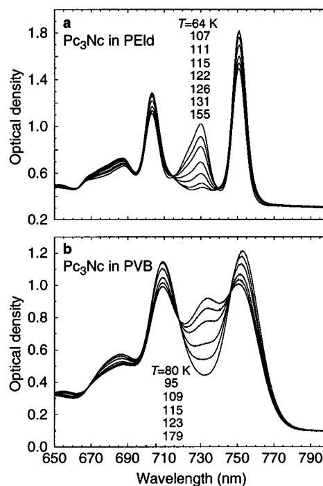
Figure 7. Temperature dependence of the absorption spectra of the photostationary mixture of NH-tautomers, produced during the exposure with white light (100 s, 100 mW/cm 2 ) at 10 K. The absorption decay of the product at 730 nm is observed as the temperature increases from the top to the bottom of the column as indicated.
