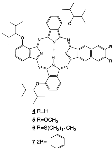
Figure 1. Chemical structure of phthalonaphthalo/anthracenocyanines \text{Pc}_3\text{NcR}_2 and \text{Pc}_3\text{An} . The configuration of protons in the stable tautomer is shown.
