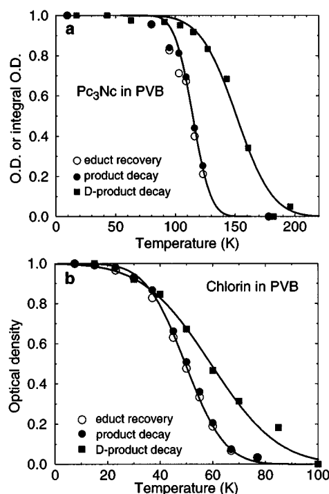
Figure 8. Normalized temperature-induced decay of the phototautomer and the recovery of educt for Pc 3 Nc (a) and chlorin (b) in PVB monitored at their respective absorption maxima. Lines are the fittings with the integrated Gaussian functions (see Figure 9).
