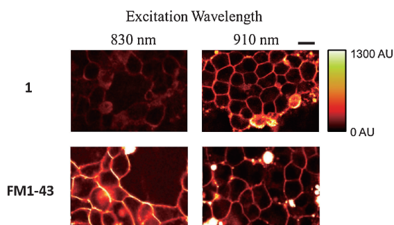
Figure 4. Two-photon excitation live images of clusters of INS-1 cells which were stained with either 1 or FM1-43 . Each dye was applied from the extracellular medium at a concentration of 10 \mu M. The excitation wavelength was 830 or 910 nm, as indicated. The fluorescence intensities were represented by the pseudocolor code (inset), where AU stands for arbitrary unit. The mean AU values of the plasma membranes at 830 nm were 200 and 2600 AU for 1 and FM1-43 , and those at 910 nm were 900 and 300 AU for 1 and FM1-43 , respectively. The scale bar indicates 10 \mu m.
