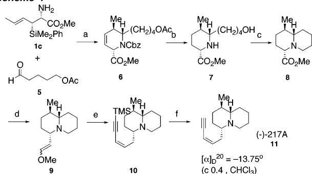
Scheme 4 a
