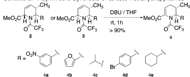
Scheme 4 a
