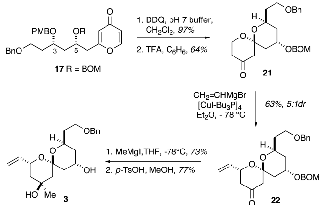
Scheme 5. Completion of AB Spiroketal
