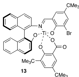
Figure 2. Carreira's catalyst.
