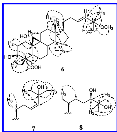
Figure 2. Significant correlations observed in the long-range ^1\text{H} – ^{13}\text{C} COSY spectrum of compounds 6 , 7 , and 8 . Compounds 7 and 8 also showed the same significant correlations in rings A–D as compound 6 .
