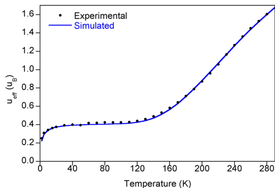
Figure 2. Variable temperature SQUID magnetization data for ( Me PDI)Fe(biphenyl) from 4 to 300 K. Data (black dots) are corrected for underlying diamagnetism, and the simulation (blue line) depicts a phase transition from an S = 0 to S = 1 state (as fit using the Sorai and Seki domain model) 49,50 with a transition temperature of 352 K and enthalpy, n\Delta H = 805 \text{ cm}^{-1} . The model also contains 0.5% of a paramagnetic impurity with \theta = -5 \text{ K} .
