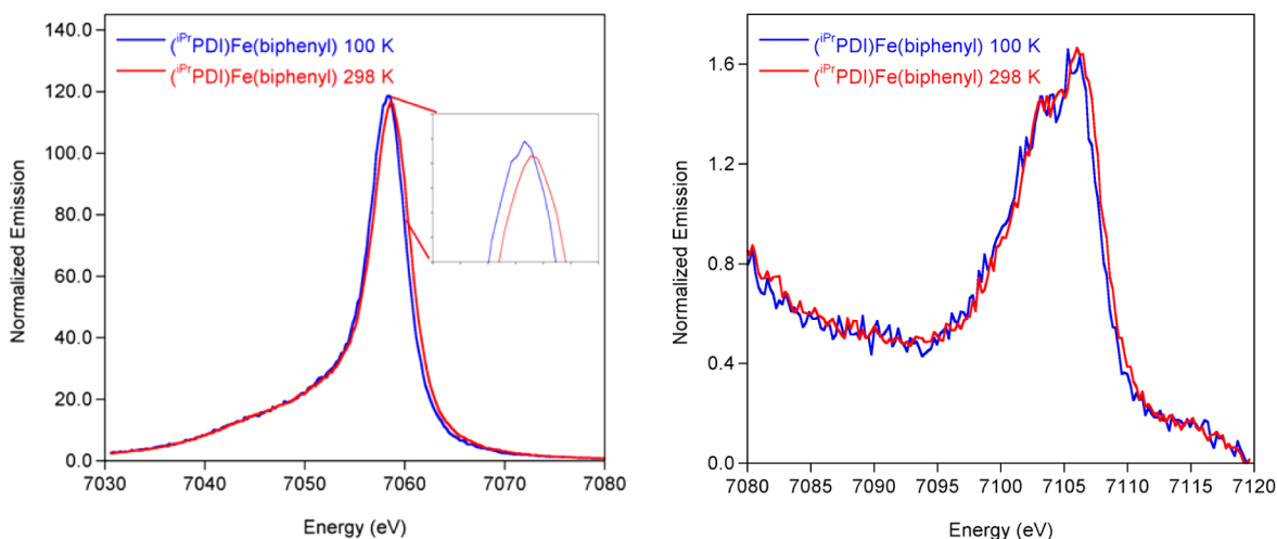
Figure 6. Variable temperature XES spectra of (i\text{PrPDI})\text{Fe}(\text{biphenyl}) highlighting the main line (left) and V2C (right) at 100 K (blue) and 298 K (red).
