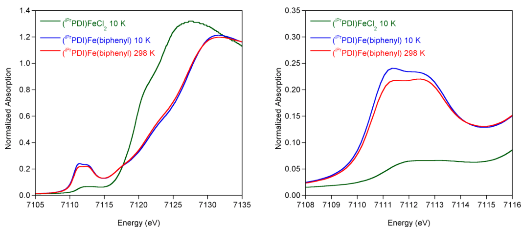
Figure 5. Comparison of the normalized Fe K-edge XAS spectra for (i\text{PrPDI})\text{FeCl}_2 and (i\text{PrPDI})\text{Fe}(\text{biphenyl}) . The data for the latter were collected at 10 (blue) and 298 (red) K. The data for (i\text{PrPDI})\text{FeCl}_2 were taken from ref 36. See Supporting Information for figures detailing the full set of experiments.
