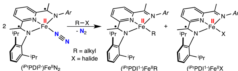
Scheme 3. C–X Oxidative Addition to (i^{\text{Pr}}\text{PDI})\text{FeN}_2 and (^{\text{Me}}\text{PDI})\text{CoN}_2
