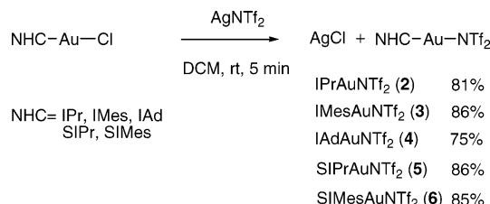
Scheme 4. Synthetic Route to (NHC)AuNTf 2 Complexes
