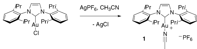
Scheme 3. NHC Gold(I) Complexes Envisaged
