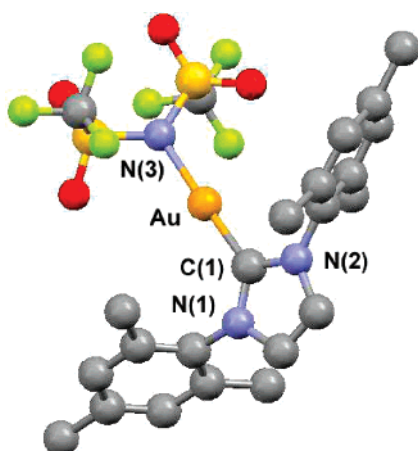
Figure 2. Molecular structure of IMesAuNTf 2 (3). Hydrogen atoms are omitted for clarity. Selected bond distances (Å) and angles (deg): Au–C(1) = 1.976(3), Au–N(3) = 2.077(2); C(1)–Au–N(3) = 177.4(1).
