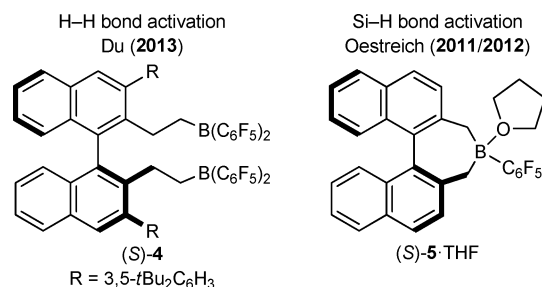
Figure 2. Axially chiral borane catalysts for the reduction of imines by hydrogenation (left) and hydrosilylation (right).
