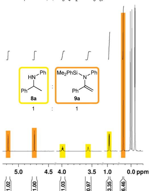
Figure 5. Segment of the 1 H NMR spectrum manifesting the equimolar ratio of free amine 8a and N -silylated enamine 9a .
