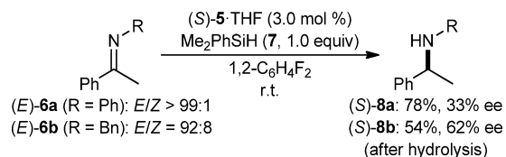
Scheme 1. Enantioselective Imine Hydrosilylations Catalyzed by ( S )- 5 ·THF
