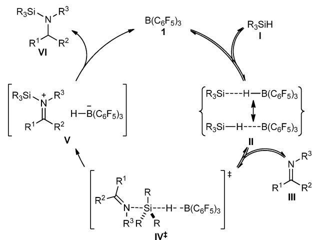
Scheme 2. Currently Accepted Mechanism of \text{B}(\text{C}_6\text{F}_5)_3 -Catalyzed Imine Hydrosilylation
