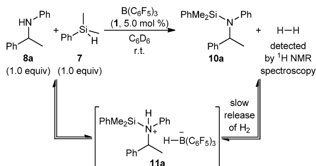
Scheme 4. B(C 6 F 5 ) 3 -Catalyzed Dehydrogenative Si–N Coupling
