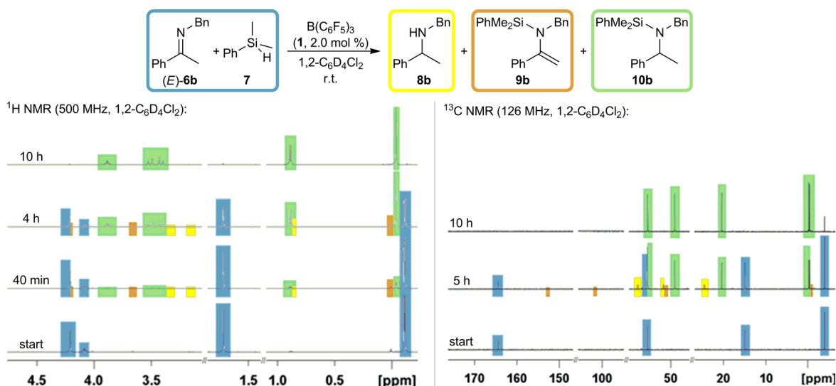
Figure 6. Time-resolved NMR studies of the B(C_6F_5)_3 -catalyzed hydrosilylation of N -benzylimine ( E )-6b.
