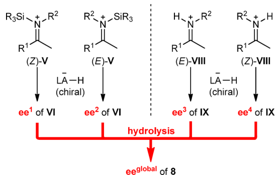
Scheme 8. Enantioselectivity-Determining Hydride Reduction of Two Pairs of Isomeric Iminium Ions Contributing to the Global Enantiomeric Excess
