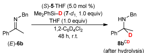
Scheme 5. Fate of the Hydride at the Silicon Atom
