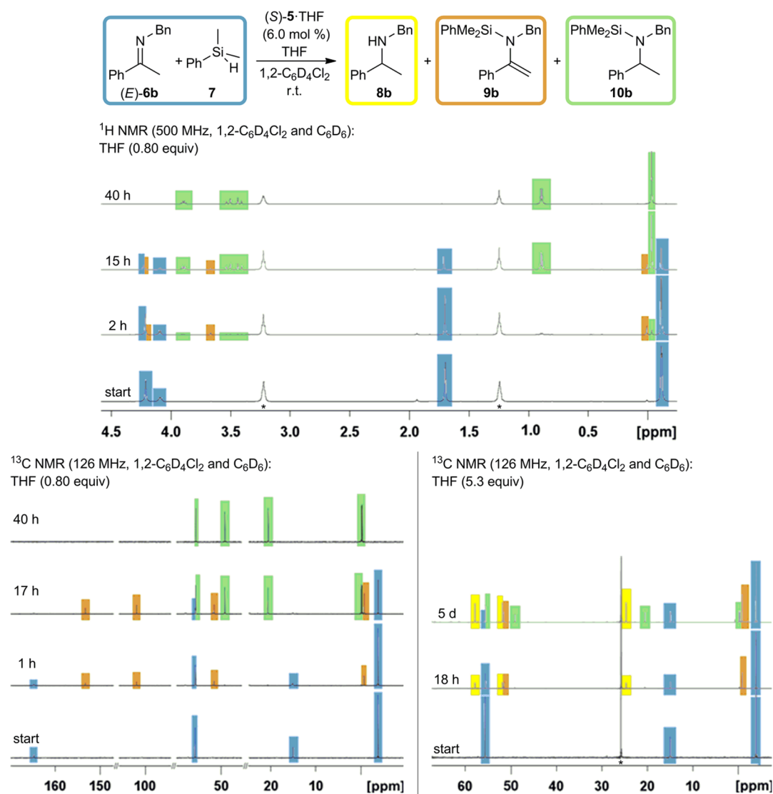
Figure 3. Effect of added THF: time-resolved NMR studies of the hydrosilylation of N -benzylated imine ( E )-6b catalyzed by ( S )-5-THF (THF indicated by asterisk).
