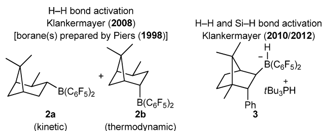
Figure 1. Terpene-derived chiral borane (pre)catalysts for the reduction of imines by hydrogenation 8a,b and/or hydrosilylation. 7a
