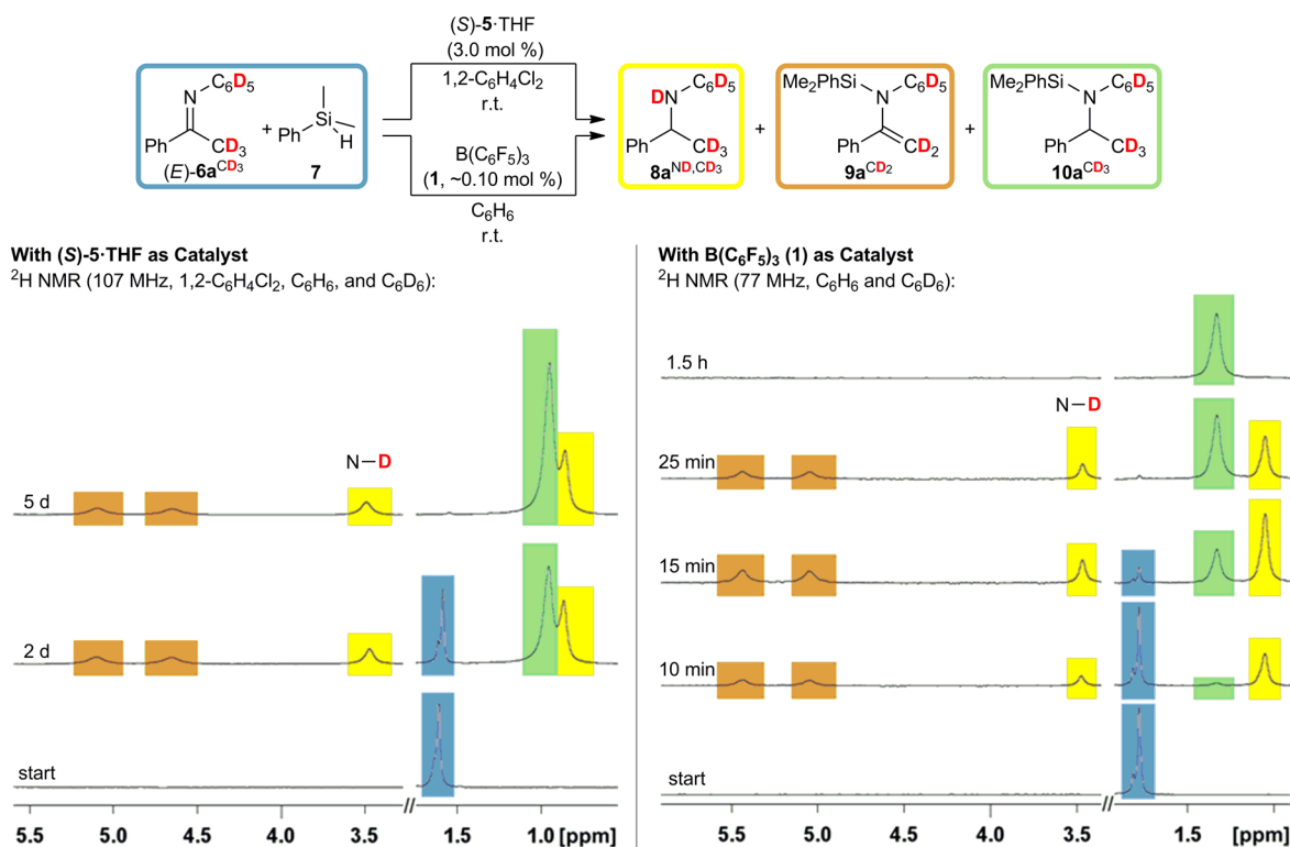
Figure 8. Time-resolved ^2\text{H} NMR studies of the hydrosilylation of deuterium-labeled N -phenylimine (E)\text{-}6\text{a}^{\text{CD}_3} catalyzed by either (S)\text{-}5\text{-THF} (left) or \text{B}(\text{C}_6\text{F}_5)_3 (1) (right): evidence for proton abstraction by unreacted (E)\text{-}6\text{a}^{\text{CD}_3} .
