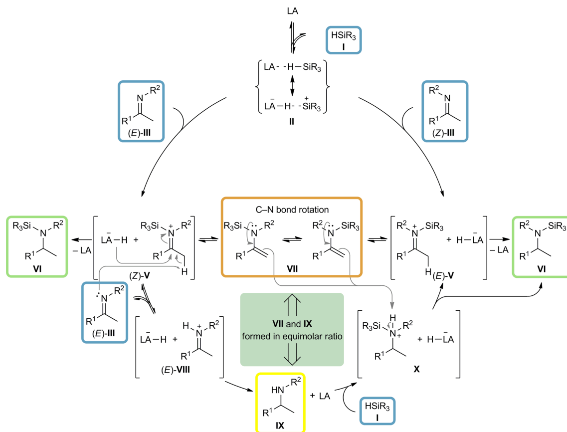
Scheme 7. Refined Mechanism of the Hydrosilylation of Imines Catalyzed by Electron-Deficient Boron Lewis Acids (One out of Four Possible Deprotonation/Protonation Scenarios Shown for the Sake of Clarity)
