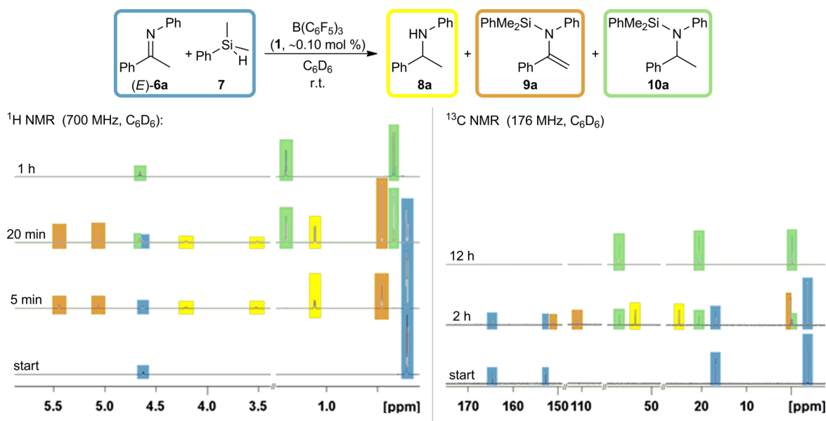
Figure 7. Time-resolved NMR studies of the B(C_6F_5)_3 -catalyzed hydrosilylation of N -phenylimine ( E )-6a.
