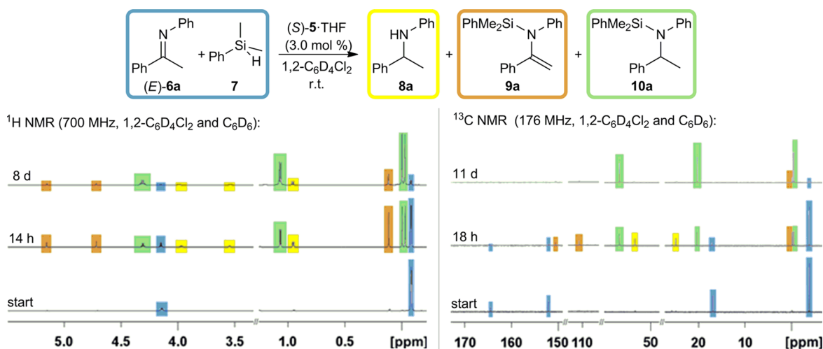
Figure 4. Time-resolved NMR studies of the hydrosilylation of N -phenylimine ( E )- 6a catalyzed by ( S )- 5-THF .
