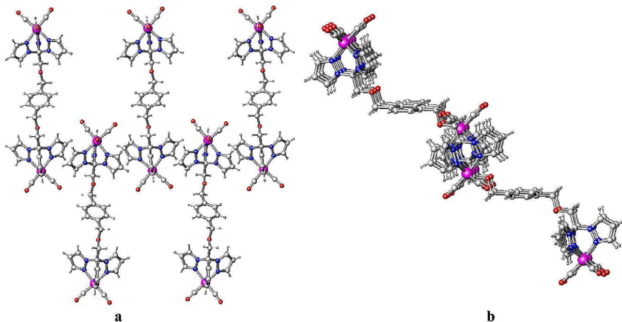
Fig. 2. The 2D sheet for 1 formed by intermolecular \pi-\pi/\text{C}-\text{H}\cdots\pi interactions: (a) view perpendicular on sheet; (b) view parallel to sheet, showing the stair-like arrangement of the sheet.
