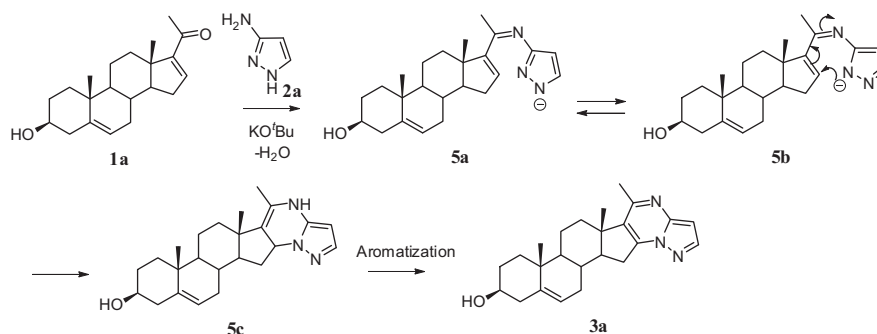
Scheme 2. Proposed mechanism for the formation of steroidal 5-methylpyrazolo[1,5- a ]pyrimidine 3a .
