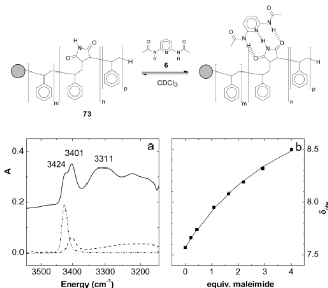
Figure 6. (a) Infrared spectra of 2,6-bis(acetylamino)pyridine 6 (dot-dashed), star 73 (dashed), and a 1:1 mixture of 6 and 73 in \text{CDCl}_3 (8 mM) (solid). (b) NMR titration curve obtained by addition of 73 to a 17 mM solution of 6 in \text{CDCl}_3 .
