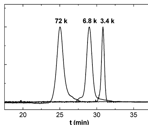
Figure 4. GPC traces for the starting dendritic initiator, 77 ( M_n = 3400 , PDI = 1.002 ), intermediate dendritic-polystyrene block copolymer, 59 ( M_n = 6800 , PDI = 1.07 ), and the final dendritic star block copolymer, 75 ( M_n = 72\,000 , PDI = 1.19 ).
