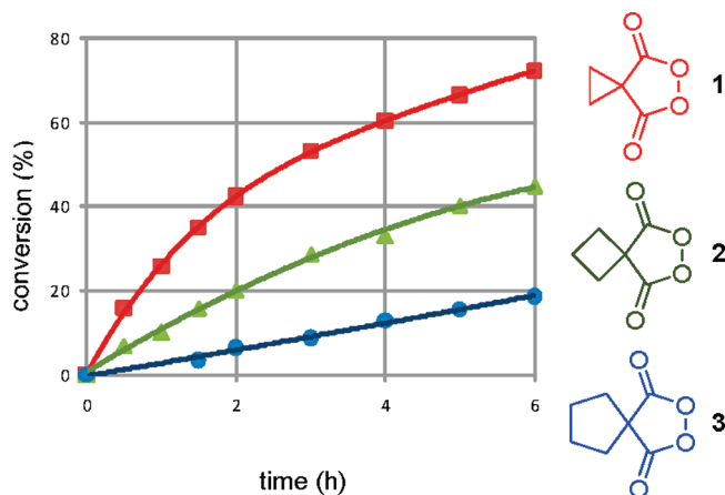
Figure 1. Relative rates for the reaction of peroxides 1–3 with styrene. All of the reactions were performed in CHCl 3 (0.6 M) at 40 °C in the presence of H 2 O (1.0 equiv). (■) peroxide 1 ; (▲) peroxide 2 ; (●) peroxide 3 .
