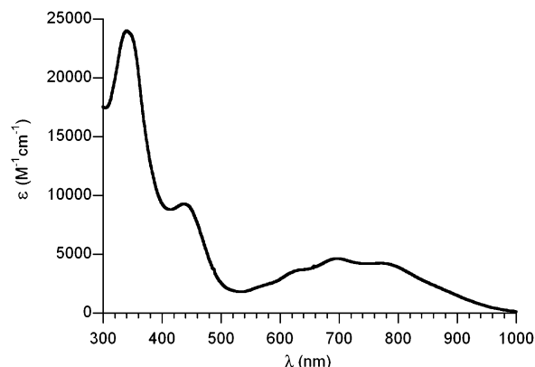
FIGURE 3. Absorption spectrum of TDC in toluene at room temperature.
