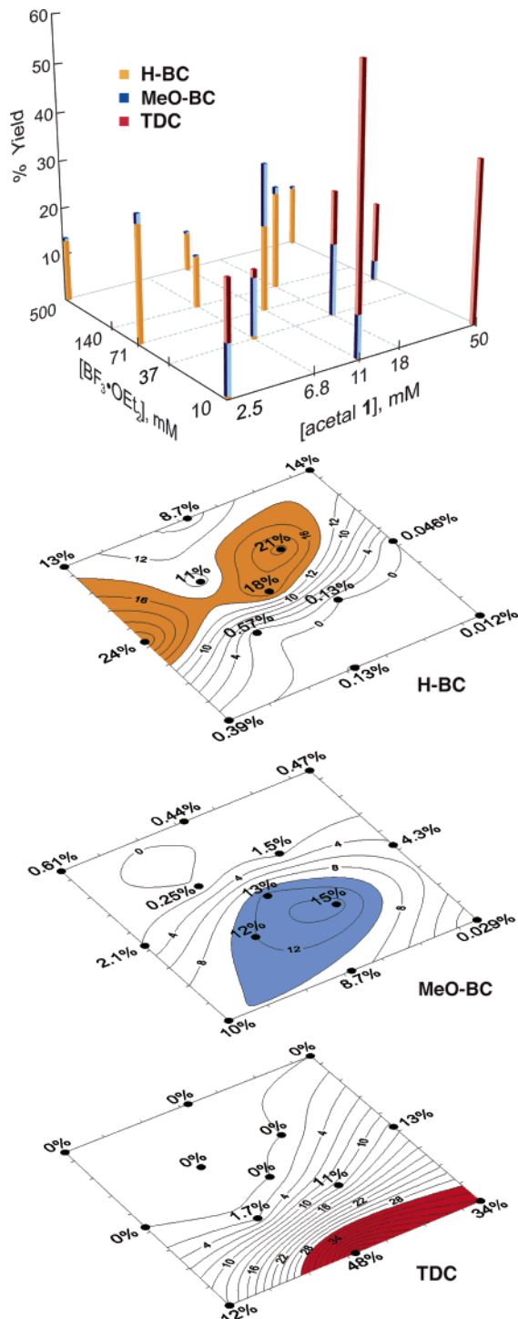
FIGURE 2. Yields of H-BC , MeO-BC , and TDC as a function of the concentrations of 1 and \text{BF}_3 \cdot \text{OEt}_2 . The reactions were performed at the microscale level. Each reaction was worked up after 23 h. The yields are based on spectrophotometry of purified fractions using the known molar absorption coefficients of each species. The segmented histogram (top) shows the yield of each species and the summed yield of macrocycles. The contour diagrams below illustrate the yield of each species H-BC , MeO-BC , and TDC in the same search space. The actual numerical data are listed; the interpolated contours are provided to guide the eye. In each contour, coloration is provided to illustrate the 60% cutset data (i.e., those regions that afford a yield that is at least 60% of the highest value recorded anywhere in the search space).
