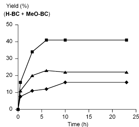
FIGURE 1. Yield of bacteriochlorins (sum of H-BC + MeO-BC ) as a function of time. The data points were taken for concentrations of 1 and \text{BF}_3 \cdot \text{OEt}_2 located along the diagonal of the grid described in Figure 2 (◆, 2.5 mM 1 , 10 mM \text{BF}_3 \cdot \text{OEt}_2 ; ■, 11 mM 1 , 71 mM \text{BF}_3 \cdot \text{OEt}_2 ; ▲, 50 mM 1 , 500 mM \text{BF}_3 \cdot \text{OEt}_2 ). The yield values were determined by absorption spectroscopy of crude reaction samples (assuming \epsilon_{\text{Qy}} = 120\,000\text{ M}^{-1}\text{ cm}^{-1} for both bacteriochlorins).
