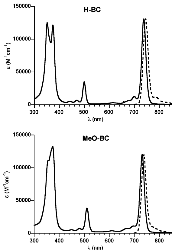
FIGURE 4. Electronic spectra of H-BC and MeO-BC in toluene at room temperature. Absorption (solid line); emission (dashed line).
