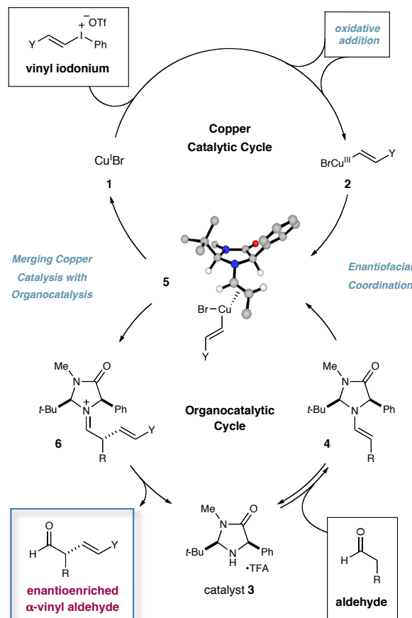
Scheme 1. Proposed Synergistic Cycles for Aldehyde \alpha -Vinylation
