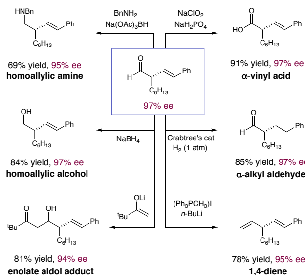
Scheme 2. Access to Diverse Enantioenriched Vinyl Synthons
