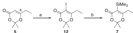
Scheme 2. (a) N -Iodosuccinimide, AcOH, room temp., 18 h, 87%; (b) Me 3 SiOTf, n -BuLi, THF, −90 °C, 10 min, 89%.
