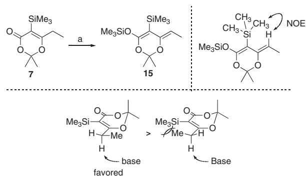
Scheme 4. (a) LiN( i -Pr) 2 , THF, −78 → −40 °C, 2 h; Me 3 SiCl, −78 °C, 1 h, 63%.
