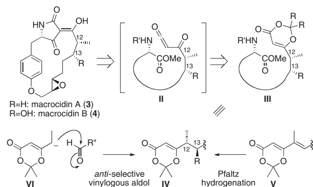
Figure 1. Retrosynthesis of the macrocadinins.
