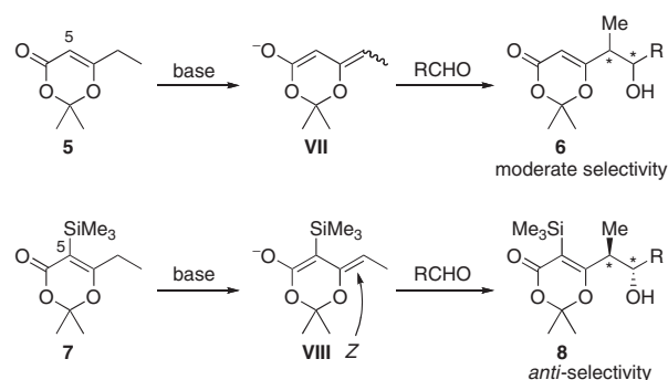
Scheme 1. Vinylogous aldol reaction.
