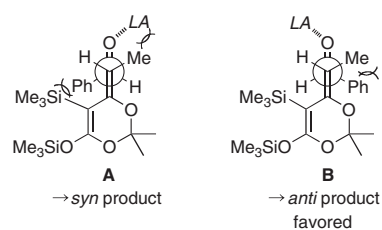
Figure 3. Transition-state model.
