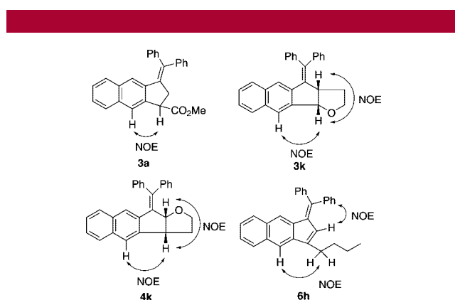
Figure 1. NOE experiment of 3a , 3k , 4k , and 6h .
