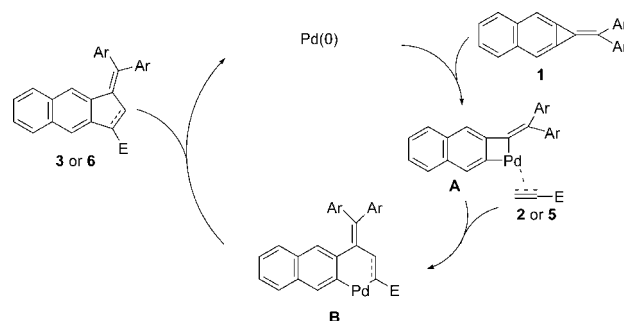
Scheme 2. Proposed Mechanism
