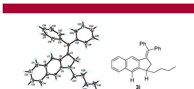
Figure 2. X-ray structure of compound 3i .
