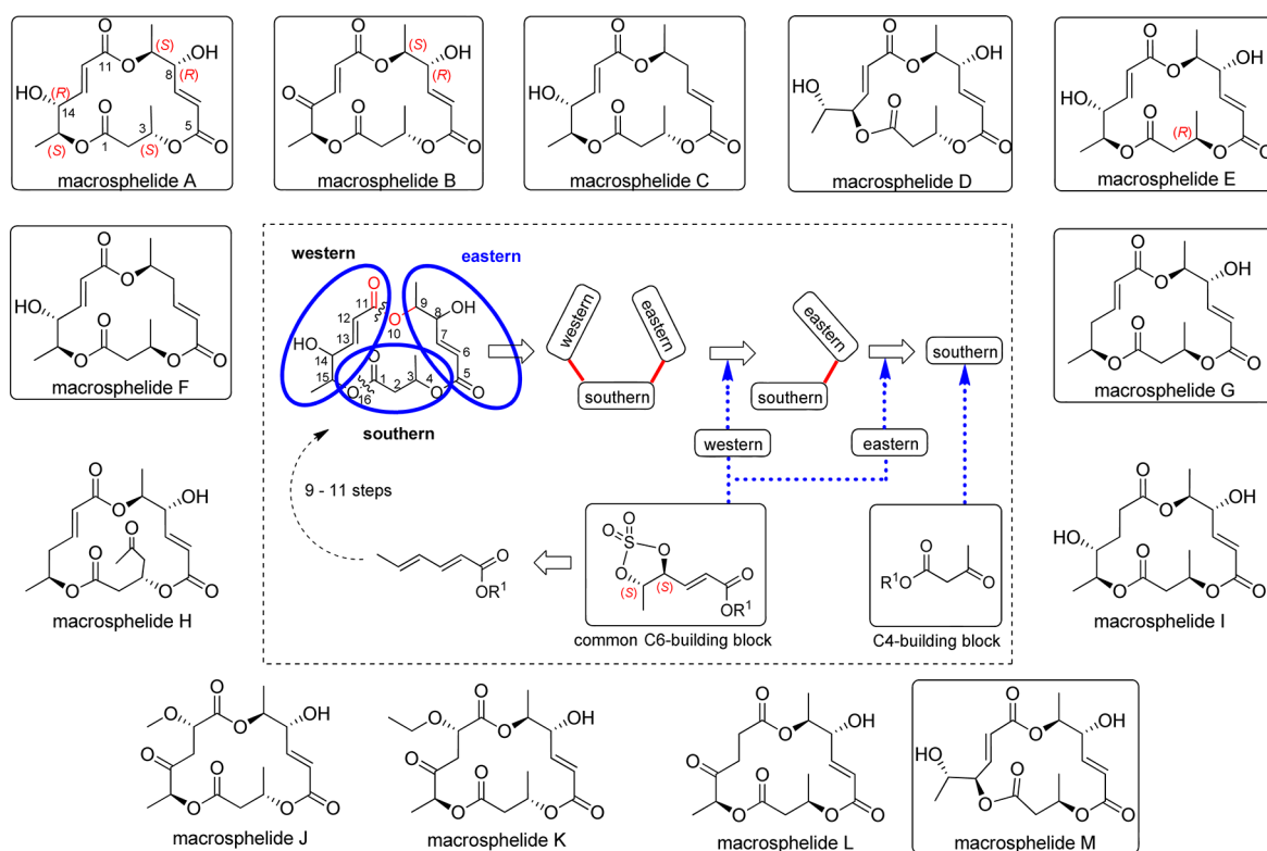
Figure 1. Macrophelide natural product family 1,2 and retrosynthetic approach.
