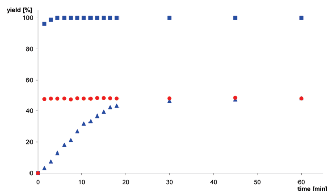
Figure 7. Metathesis of 1-phenyl-1-propyne catalyzed by Mo(≡CPh)(OSiPh 3 ) 3 (Et 2 O) ( 24 ⋅Et 2 O, 1 mol %) in toluene in the absence (blue triangles) or in the presence (blue squares) of powdered MS 5 Å at ambient temperature. Comparison with the plot obtained upon pretreatment of the catalyst with MS 5 Å, which was removed prior to the addition of the substrate (red circles). The yields were measured by GC against biphenyl as internal standard.
