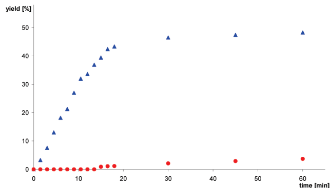
Figure 4. Metathetic conversion of 1-phenyl-1-propyne to tolane catalyzed by 1 mol % of either \text{Mo}(\equiv\text{CPh})(\text{OSiPh}_3)_3(\text{Et}_2\text{O}) ( 24 ⋅ \text{Et}_2\text{O} ) (blue triangles) or (t\text{BuO})_3\text{W}\equiv\text{CtBu} ( 1 ) (red circles) in toluene at ambient temperature and ambient pressure. The yields were determined by GC using biphenyl as an internal standard.
