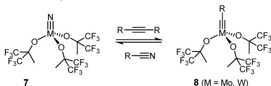
Scheme 2. Metal Nitride/Metal Alkylidyne Interconversion as an Alternative Concept for the in Situ Generation of Alkyne Metathesis Catalysts a
