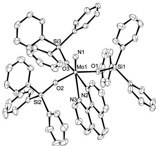
Figure 1. Structure of \text{Mo}(\equiv\text{N})(\text{OSiPh}_3)_3(\text{phen}) ( 15 ) in the solid state ( \text{N1-Mo1-N2} = 91.2(1)^\circ ). Disordered solute toluene is omitted for clarity; phen = 1,10-phenanthroline.
