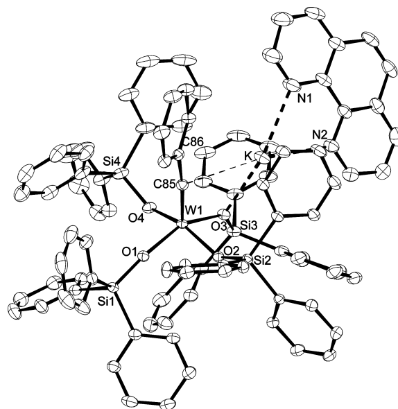
Figure 6. Structure of the ate-complex [(Ph 3 SiO) 4 W≡CPh] − [K + ⋅(phen)] ( 29 ) in the solid state.
