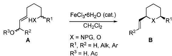
Scheme 1. FeCl 3 -Catalyzed Cyclization of \zeta -Amino and \zeta -Hydroxy Allylic Alcohol Derivatives (PG = Protective Group)
