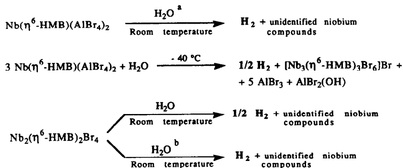
Scheme 1. a pH ca zero after decomposition of \text{Nb}(\eta^6\text{-HMB})(\text{AlBr}_4)_2 . b pH ca zero by addition of hydrobromic acid.
