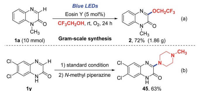
Scheme 2 Gram-scale synthesis and the synthesis of histamine-4 receptor antagonist.
