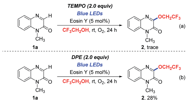
Scheme 4 Mechanism studies.
