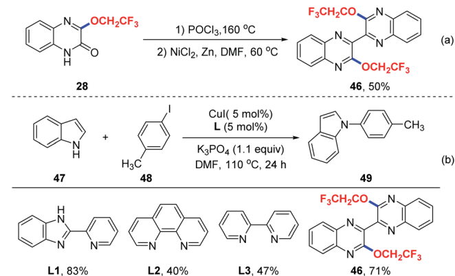
Scheme 3 Further chemistry.
