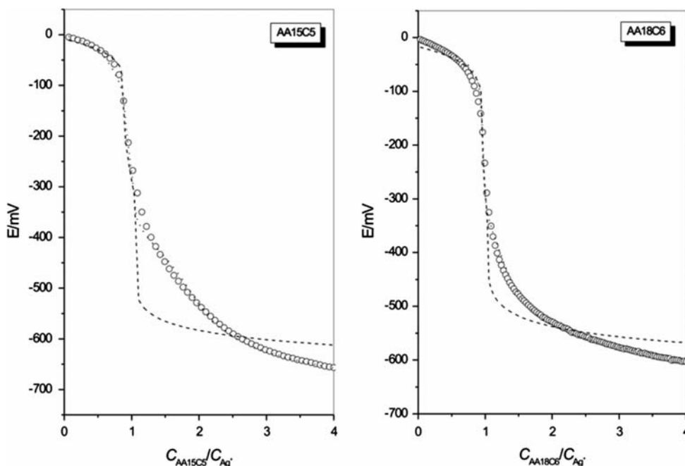
Figure 3. Graphical fitting for models 1° (—) and 2° (---) and experimental points (o) of silver(I) ( 6.00 \times 10^{-4} \text{ M dm}^{-3} ) from potentiometric titration with AA15C5 ( 4.00 \times 10^{-3} \text{ M dm}^{-3} ; left) and AA18C6 ( 4.00 \times 10^{-3} \text{ M dm}^{-3} ; right) in PC at 25 °C.
