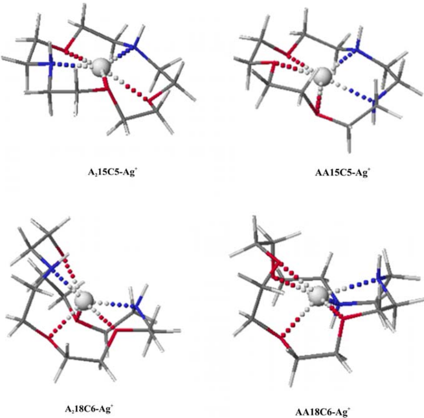
Figure 5. The most favorable structures of the 1 : 1 metal-to-ligand complexes with Ag + cations and diaza-crown ethers.
