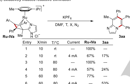
Scheme 5. X-ray crystal structure analysis and applications. Selected bond lengths [Å]: Ru-II : Ru1-N1: 2.086(3), Ru1-C3: 2.083(3), N1-C1: 1.340(4), C1-C2: 1.446(4), C2-C3: 1.356(4); Ru-IVa : Ru1-N1: 2.101(2), Ru1-C14: 2.172(3), Ru1-C15: 2.171(3), Ru1-C16: 2.222(3), N1-C13: 1.326(4), C12-C13: 1.481(4), C12-C14: 1.577(4), C12-C16: 1.564(4), C14-C15: 1.442(4), C15-C16: 1.449(4); Ru-IVb : Ru1-N1: 2.094(3), Ru1-C13: 2.220(3), Ru1-C14: 2.185(3), Ru1-C15: 2.174(3), N1-C11: 1.333(4), C11-C12: 1.477(4), C12-C13: 1.557(4), C12-C15: 1.587(4), C13-C14: 1.446(5), C14-C15: 1.449(5).
