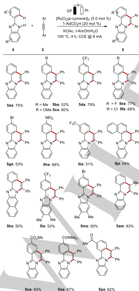
Scheme 3. Electrooxidative C–H activation of benzimidazoles 4 .
