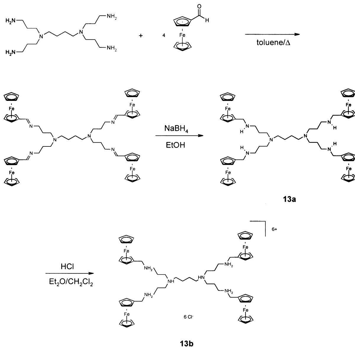
Scheme 4. Synthesis of 13b , images of 14b , 15b , 16b and 17b .
