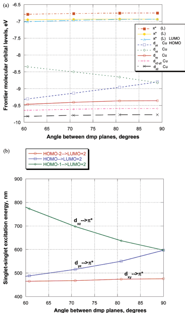
Figure 5. Top: Energy of the frontier orbitals of [Cu I (dmp) 2 ] + as a function of the angle between the dmp planes. Bottom: Excitation energies from TD-DFT calculations.
