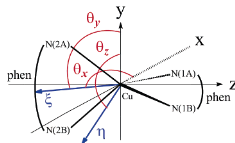
Figure 1. Schematic representation of the distortions around the copper center in Cu(II)(dmp) 2 + complexes. The \theta_x and \theta_y angles describe the rocking distortion, and \theta_z the flattening distortion. The coordinate system is chosen so that triangle N1A–Cu–N1B lies in the XZ plane. Unit vector \xi bisects angle N2A–Cu–N2B, and unit vector \eta is perpendicular to triangle N2A–Cu–N2B. \theta_x is the angle between \xi and X. \theta_y is the angle between \xi and Y. \theta_z is the angle between \eta and Y.
