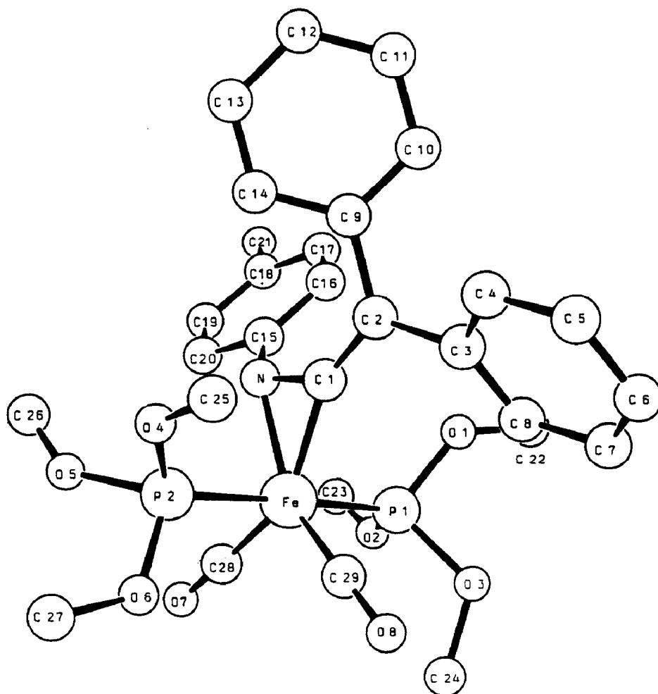
Fig. 2. Molecular structure of \text{Fe}(\text{CO})_2[\text{P}(\text{OMe})_3]_2\text{Ph}_2\text{C}_2\text{N-}p\text{-tolyl} ( 3 ) (molecule 1).
