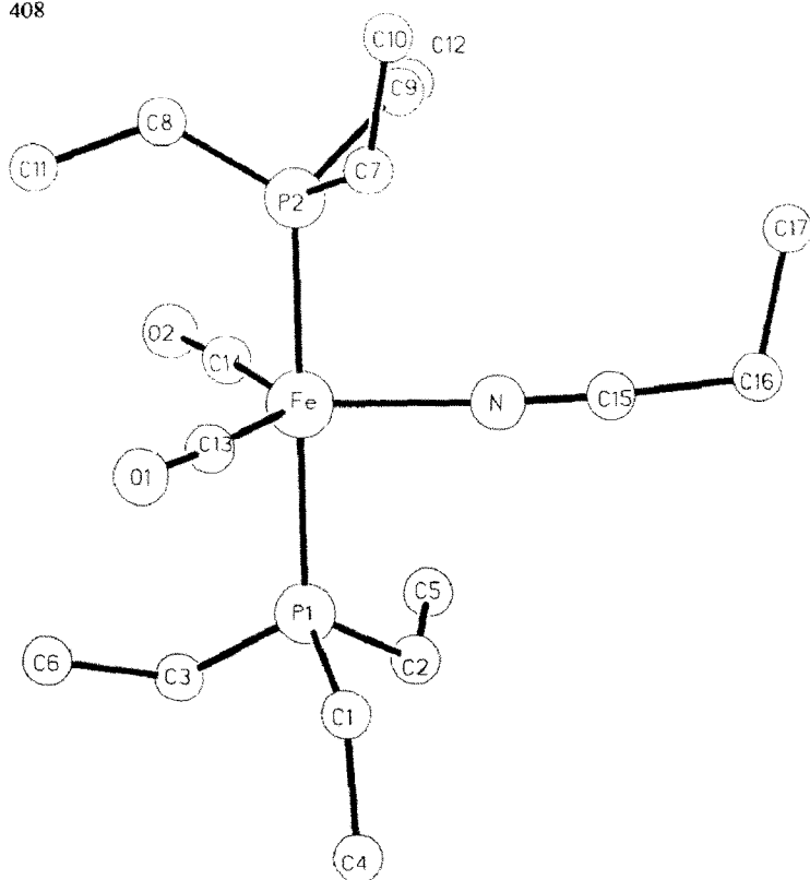
Fig. 3. Molecular structure of \text{Fe}(\text{CO})_2[\text{PEt}_3]_2\text{EtCN} ( 5a ).
