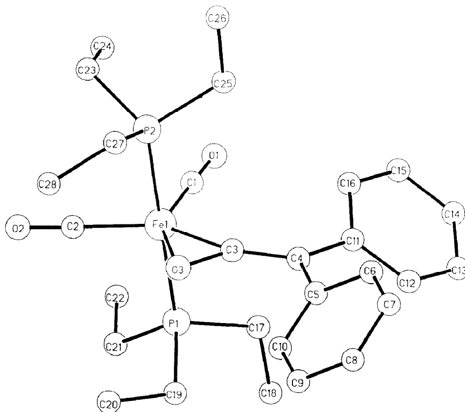
Fig. 1. Molecular structure of \text{Fe(CO)}_2[\text{PEt}_3]_2\text{Ph}_2\text{C}_2\text{O} ( 2c ).
