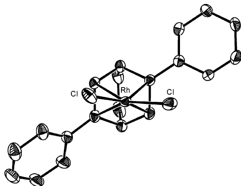
FIGURE 1. ORTEP illustration of [\text{RhCl}((S,S)\text{-Ph-bod}^*(\mathbf{3b}))_2] with thermal ellipsoids drawn at the 50% probability level (shown as a monomer for clarity). The ORTEP for the whole dimeric molecule is shown in the Supporting Information.
