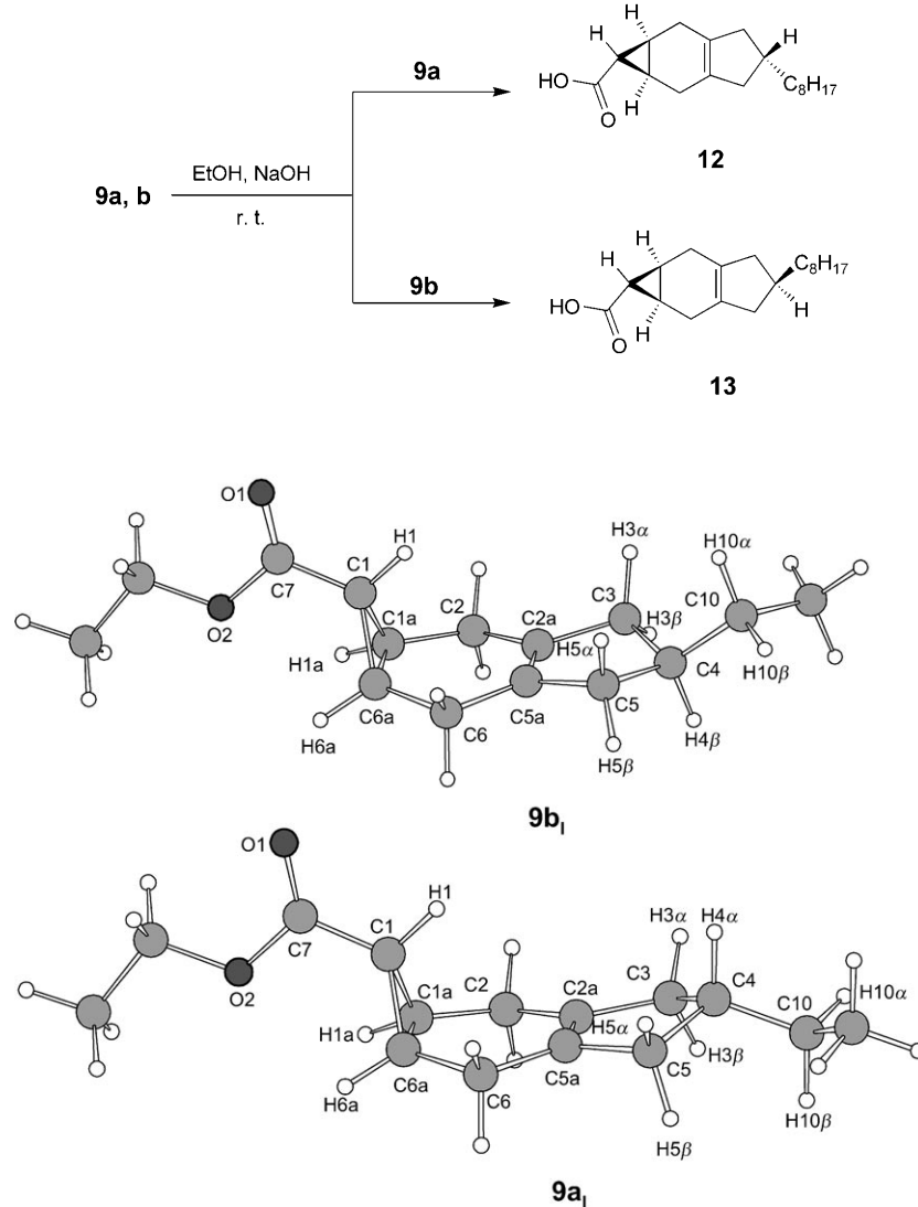
Fig. 3. B3LYP/6-31+G** optimized model structures 9a 1 and 9b 1 with a 4-ethyl group instead of the 4-octyl group
