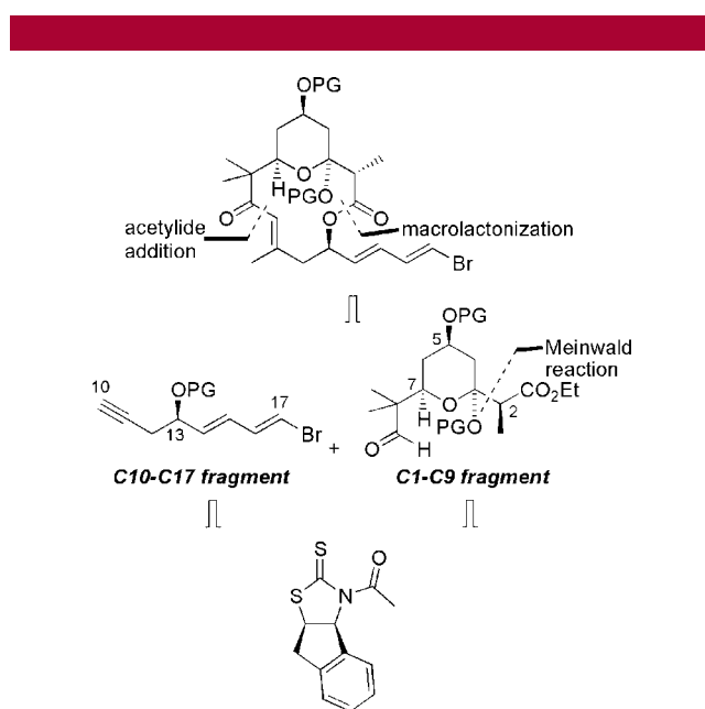
Figure 2. Retrosynthesis of the aglycon core.
