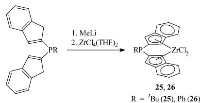
Scheme 17
