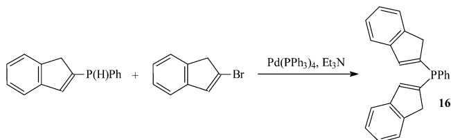
Scheme 13
