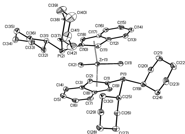
Figure 3. Crystal structure of 22 . Displacement ellipsoids are shown at the 50% probability level. Hydrogen atoms are omitted for clarity. Selected bond lengths (Å) are Zr(1)—Cl(1) 2.4132(7), Zr(1)—Cl(2) 2.4178(7), Zr(1)—C(1) 2.518(2), Zr(1)—C(2) 2.455(2), Zr(1)—C(3) 2.562(2), Zr(1)—C(8) 2.610(2), Zr(1)—C(9) 2.554(2), Zr(1)—C(10) 2.543(2), Zr(1)—C(11) 2.472(3), Zr(1)—C(12) 2.578(2), Zr(1)—C(17) 2.594(2), Zr(1)—C(18) 2.560(2), P(1)—C(1) 1.838(2), P(1)—C(19) 1.873(3), P(1)—C(25) 1.866(2), P(2)—C(10) 1.836(3), P(2)—C(31) 1.862(3), P(2)—C(37) 1.86(2), P(2)—C(37') 1.900(17).
