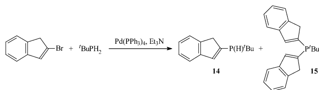
Scheme 10
