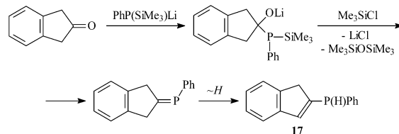
Scheme 13
