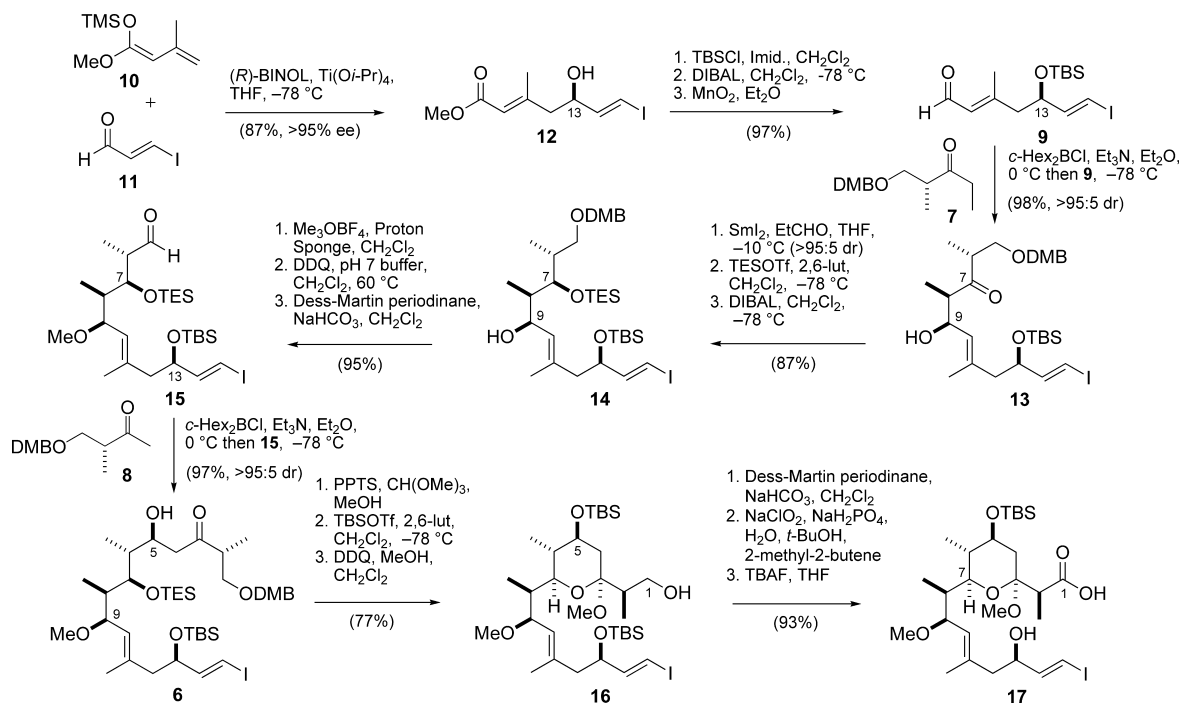
Scheme 2
