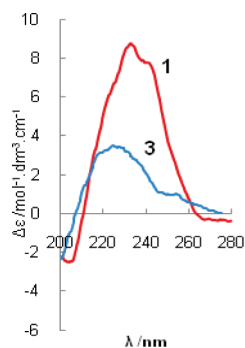
Figure 2. CD spectra in MeOH of synthetic compounds 1 , [ \alpha ] D = +53.5 ( c = 0.2, MeOH) cf. lit. +38 ( c = 0.06, MeOH), and 3 , with peak maxima compared to that of natural (+)-phorboside A.
