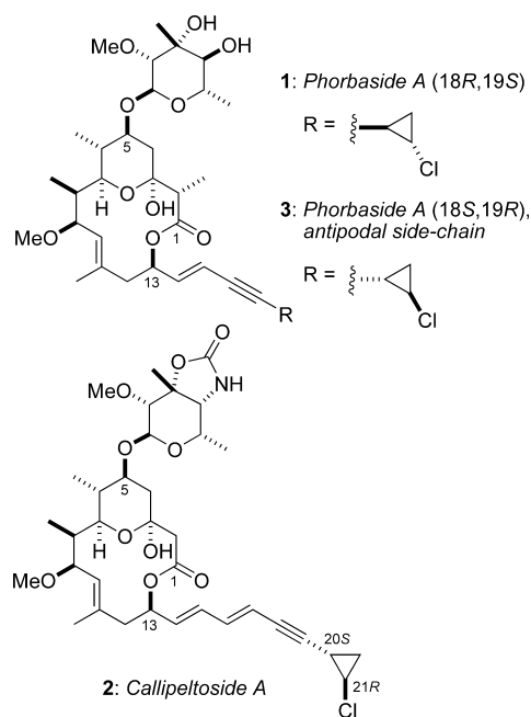
Figure 1. Phorbaside and callipeltoside marine macrolides.
